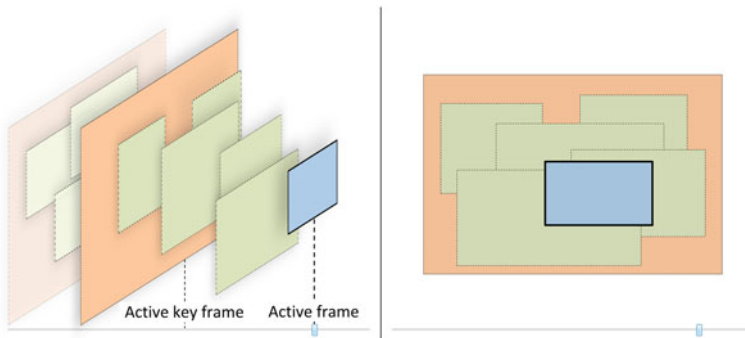
Fig. 5 Screen construction with key frames and segments
