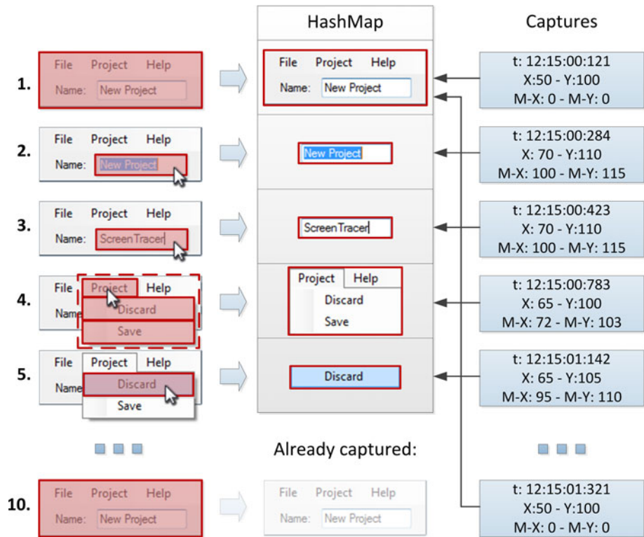
Fig. 2 Output-driven capturing of changed screen segments
