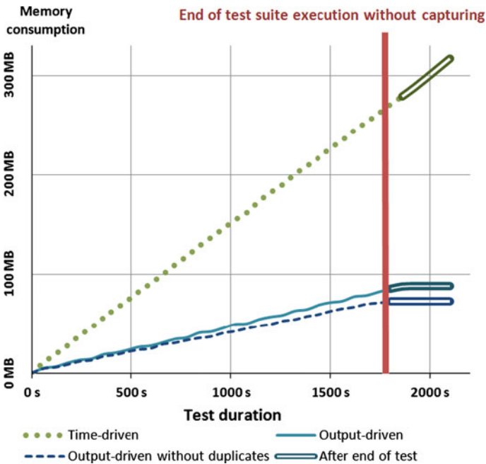
Fig. 7 Memory usage while running a representative test suite of 44 real industry test cases
