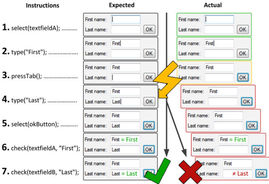
Fig. 1 Deviation of actual behavior from required behavior
