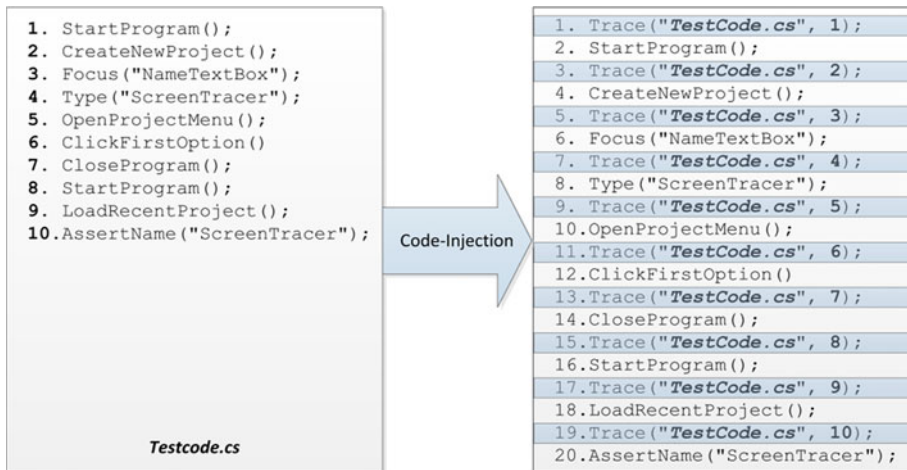
Fig. 3 Weaving of cross-cutting concern “logging” on line basis
